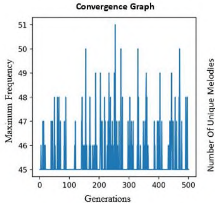
Figure 4. Convergence Graph
